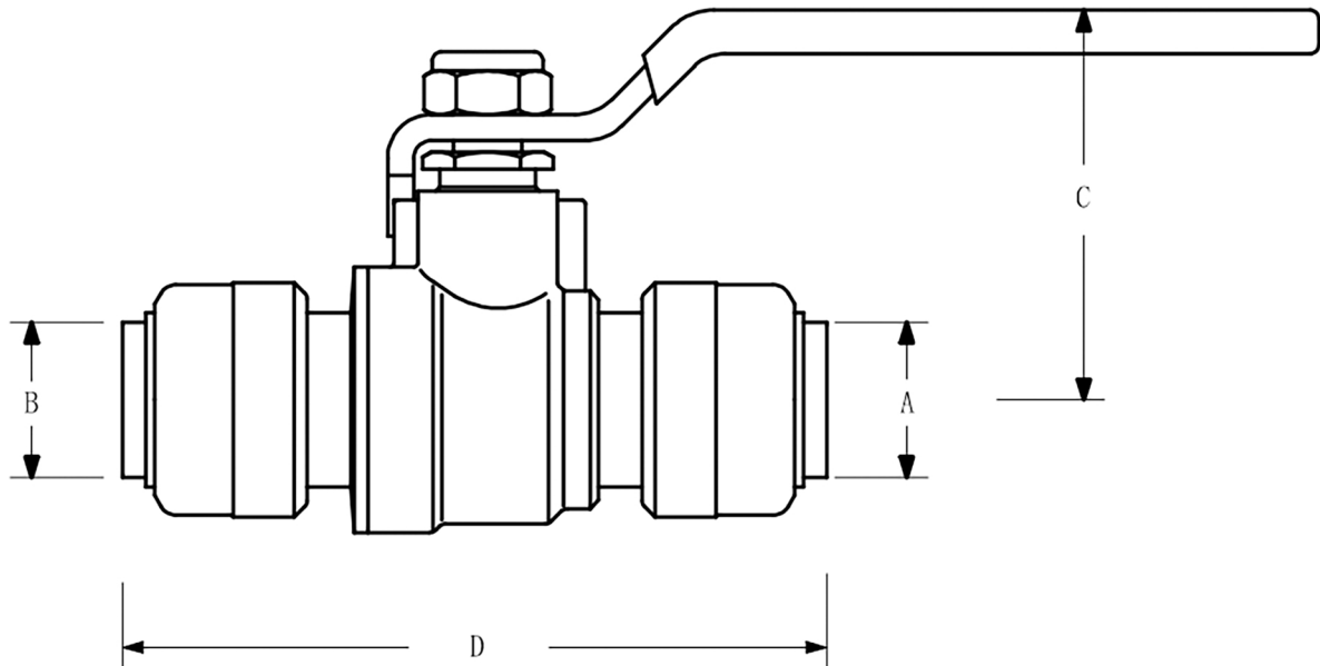
Push-Fit Ball Valves Dimensions
