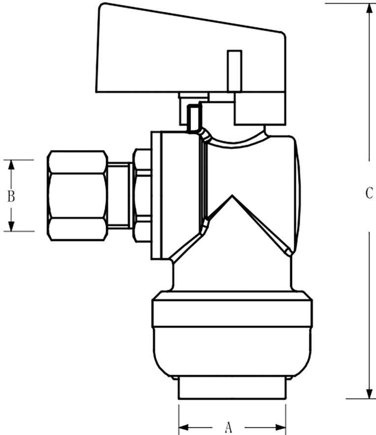
1/4Turn Angle Stop Valve
