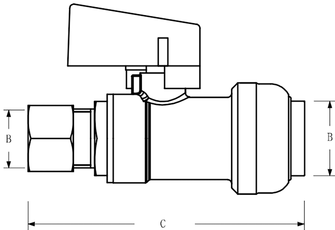
1/4Turn Straight Stop Valve
